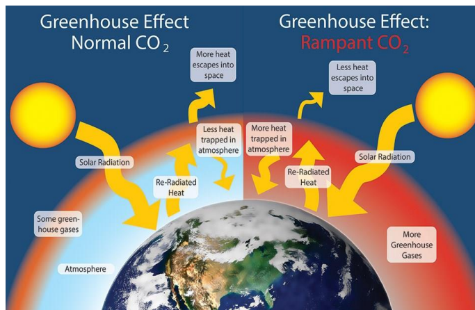
Figure 1: Visual depiction of the greenhouse effect (Yonkers, 2021)
