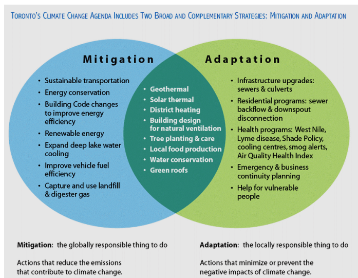
Figure 2: The overlap between mitigation and adaptation (Kazmierczak & Carter, 2010)
